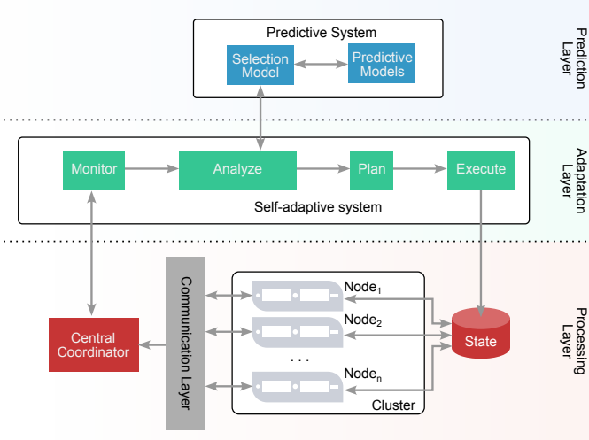
Figure 2: MMP-SPS's Architecture.
