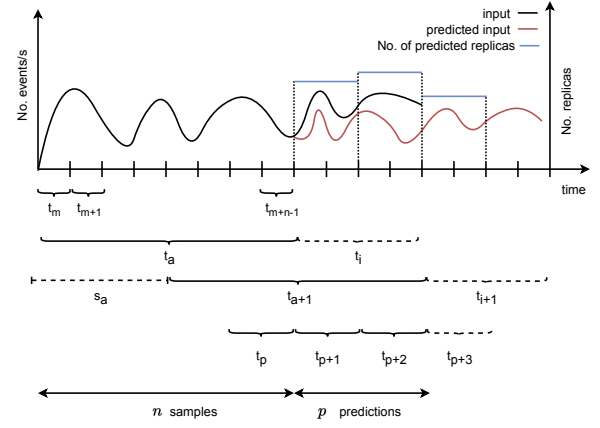
Figure 3: Example of the time windows scheme implemented by the adaptation layer
