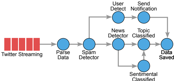
Figure 6: Social Network Application for Information Classification (IC).
