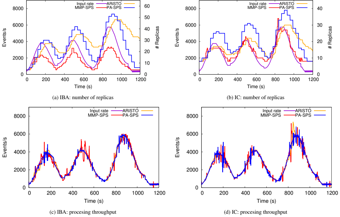
Figure 8: Performance metrics on social network scenario with IBA and IC comparing MMP-SPS, ARiSTO, and PA-SPS.
