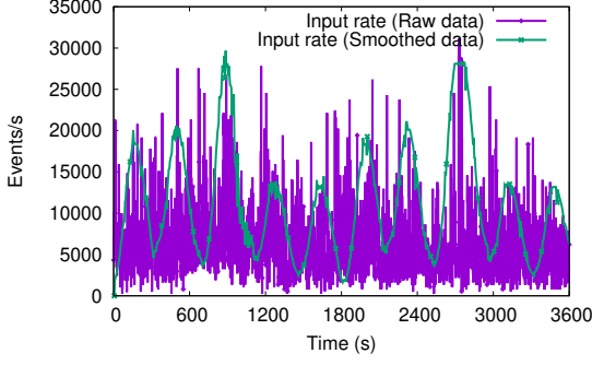
Figure 4: Traffic shape of Covid Social network dataset.
