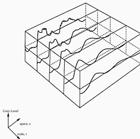
Figure 2: From [Witkin, 1983]
