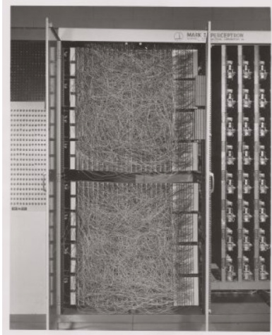
inputs weights
