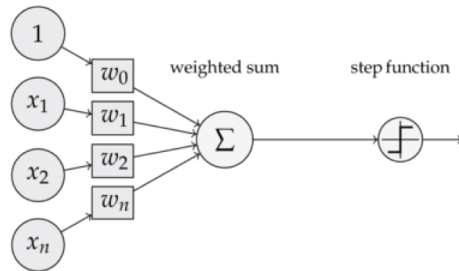
inputs weights
