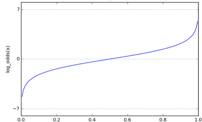
Log Odds
