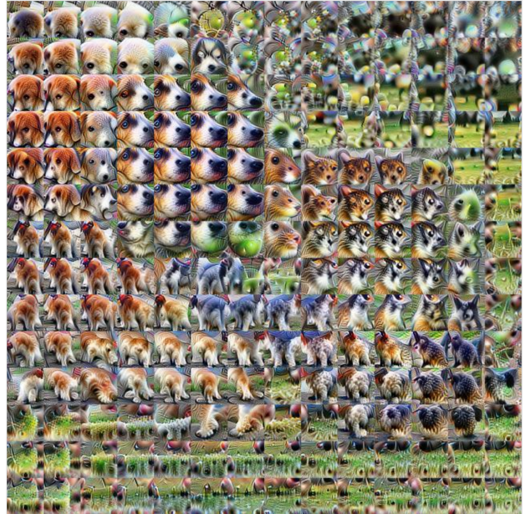
Activation grid from InceptionV1, layer mixed4d.
