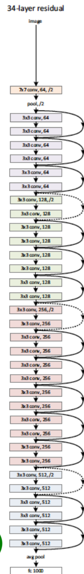
ResNet (2015)
