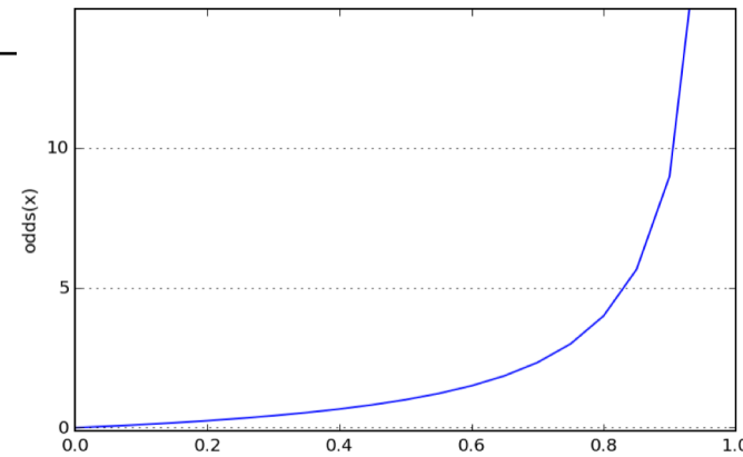
Odds
