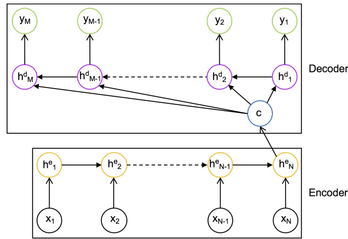
Figure 37: RNN Encoder-Decoder architecture. Inspired from [3]. The hidden layer h_t^e of the RNN encoder acts as a memory which iteratively accumulates information about the successive elements x_t of an input sequence read by the RNN encoder; resulting in a final state h_N^e ; which is passed to the RNN decoder as the summary c of the whole input sequence; which then iteratively generates the output sequence by predicting the next item y_t given its hidden state h_t^d and the summary c as a conditioning additional input
