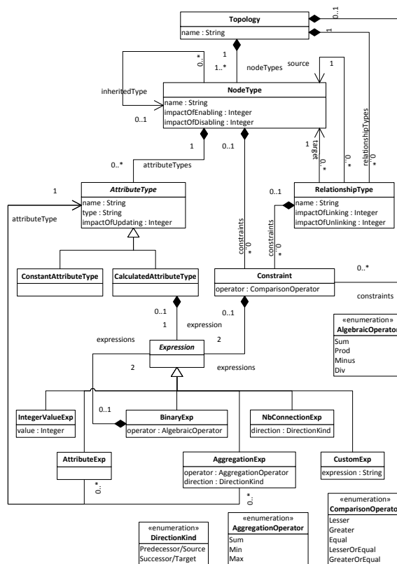
Figure 4: Topology metamodel - Design time.
