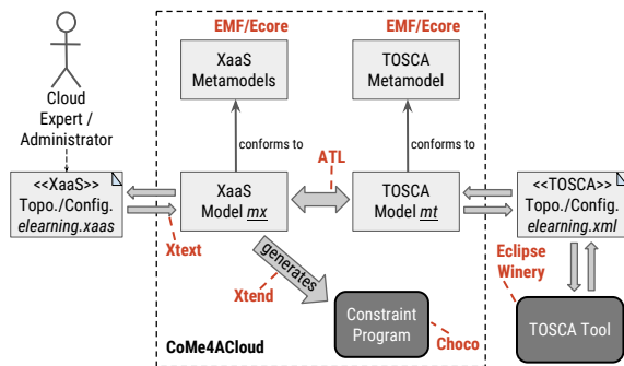
Figure 6: An Eclipse/EMF-based implementation.
