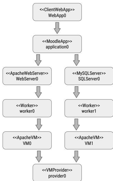
Figure 9: A reconfiguration from our motivating example (SaaS level).
