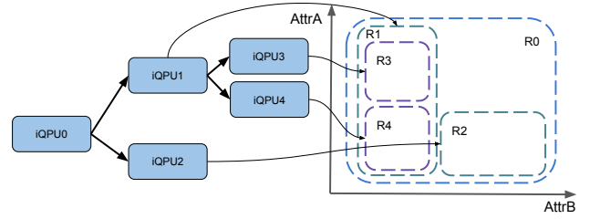
Figure 1: An example of hyperspace partitioning using an index QPU hierarchy.
