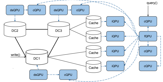
Figure 2: A QPU network configuration for querying in a content delivery network.
