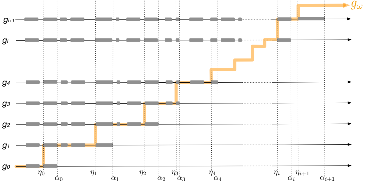
Fig. 1. Construction of (g_n)_{n \in \mathbb{N}} in the proof of Theorem 2. Grey bold lines represent instants where e belongs to the graph outputted by all process of V .
